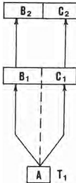
Fig. 3. Schematic diagram of the formation of paraprovincialism in the Recent Caribbean. A = ancestral species at time T 1 ; B 1 , C 1 = components of descendant ancestroma at time T 0 (Pliocene); B 2 , C 2 = descendant species pair at time T n (Recent). Dashed line between members of ancestroma represents paleoprovincial boundaries; solid line between Recent species pair represents sharp break in distributions.
