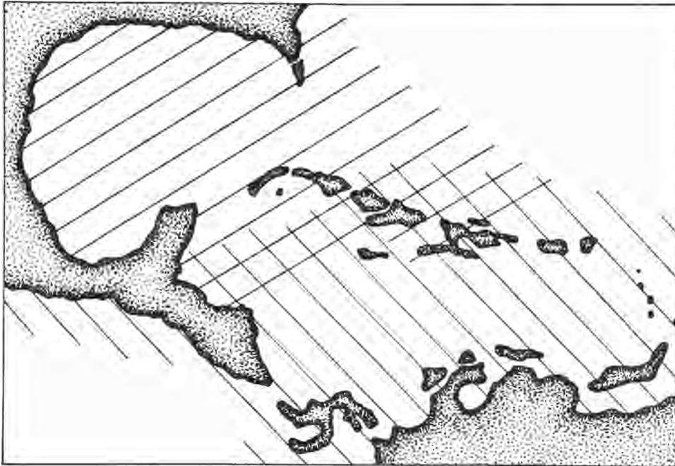
Fig. 2. Map of the Caribbean region in the Pliocene showing the distributions of the Gatunian Province (oblique lines rising to the left) and Caloosahatchian Province (oblique lines rising to the right) (after Petuch 1982).
